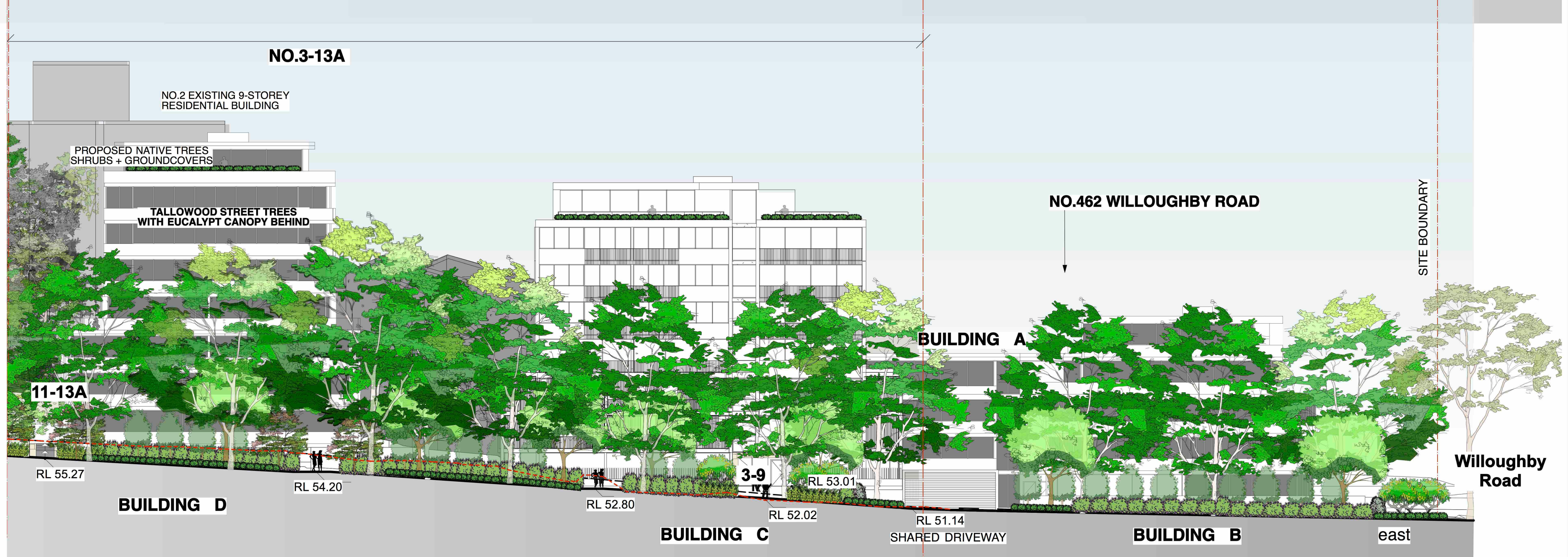
A WALTER STREET SOUTH ELEVATION 1:200
